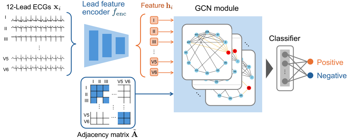
Fig. 1. Overview of the proposed method. The 12-lead ECG signals are processed by a lead feature encoder f_{\text{enc}} to extract features \mathbf{h}_i , which serve as nodes in the GCN module. The adjacency matrix \tilde{\mathbf{A}} = \mathbf{A} + \mathbf{I} defines inter-lead relationships, and the GCN output is fed to a CTRCD classifier.
